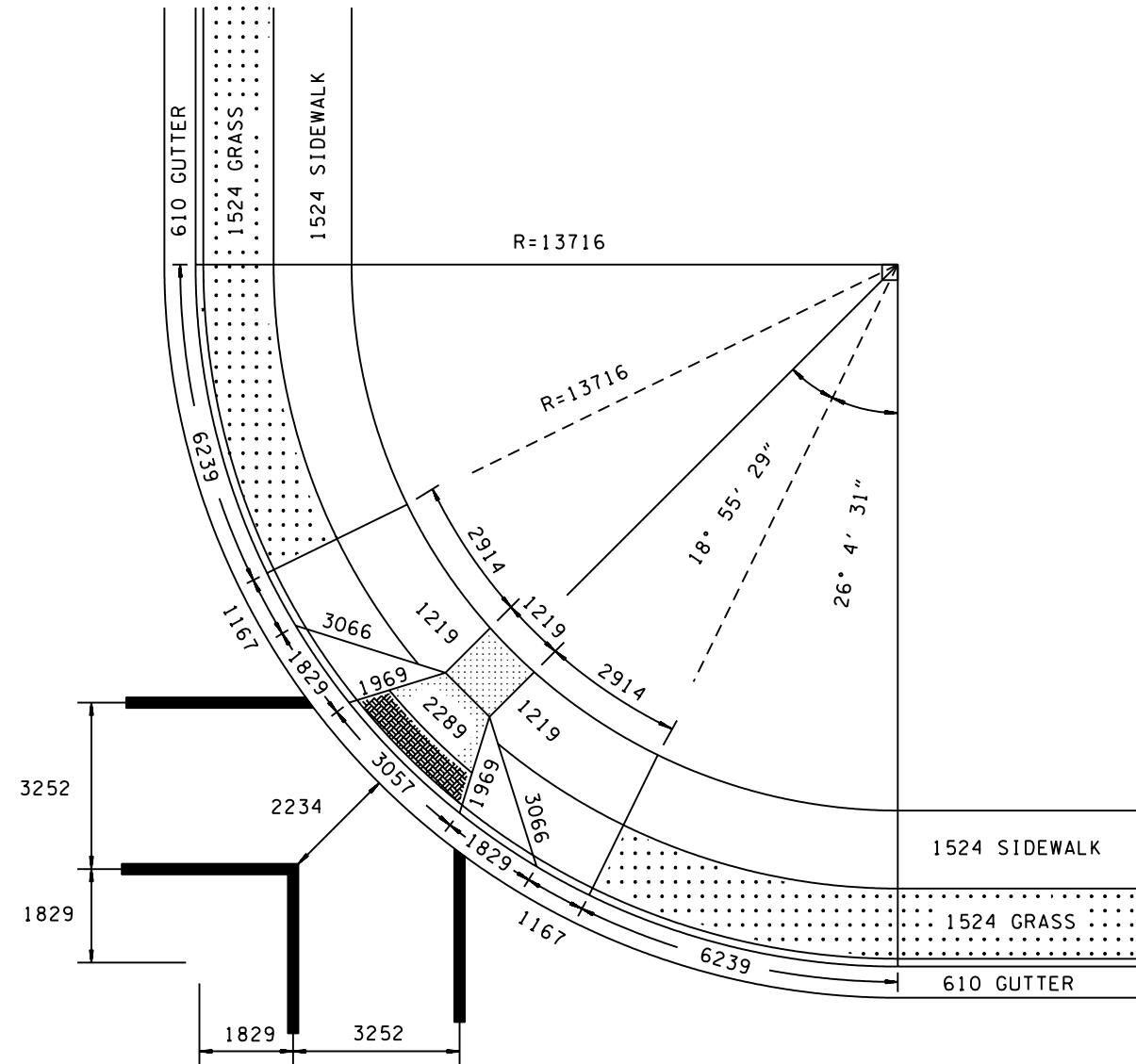
WITH 1524 mm GRASS STRIP R=13716
