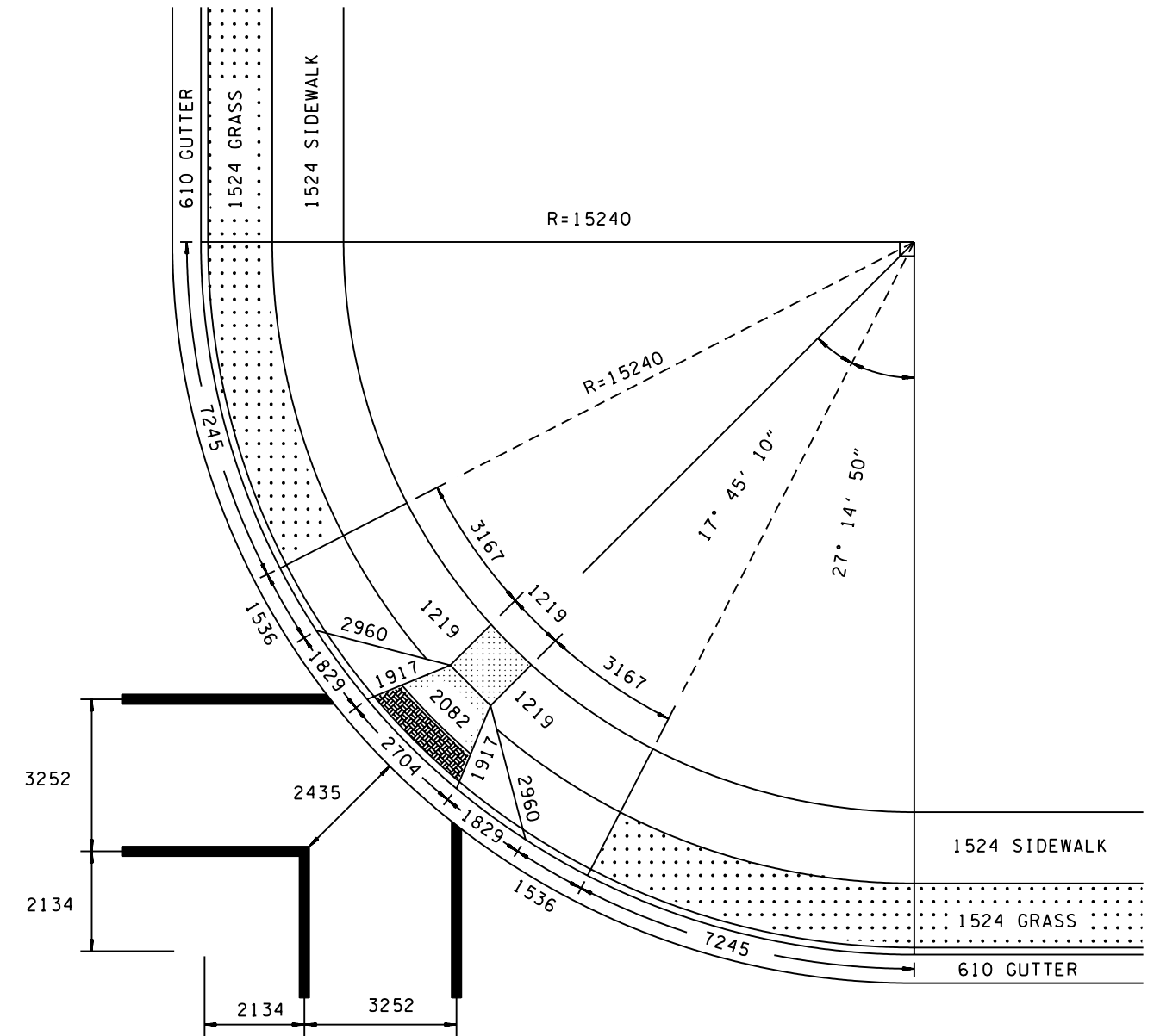
WITH 1524 mm GRASS STRIP R=15240
